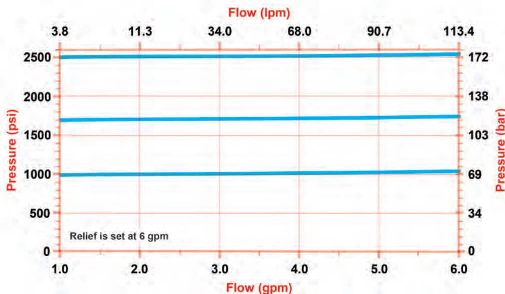
Pressure VS. Flow for Pilot Relief (DCF)
