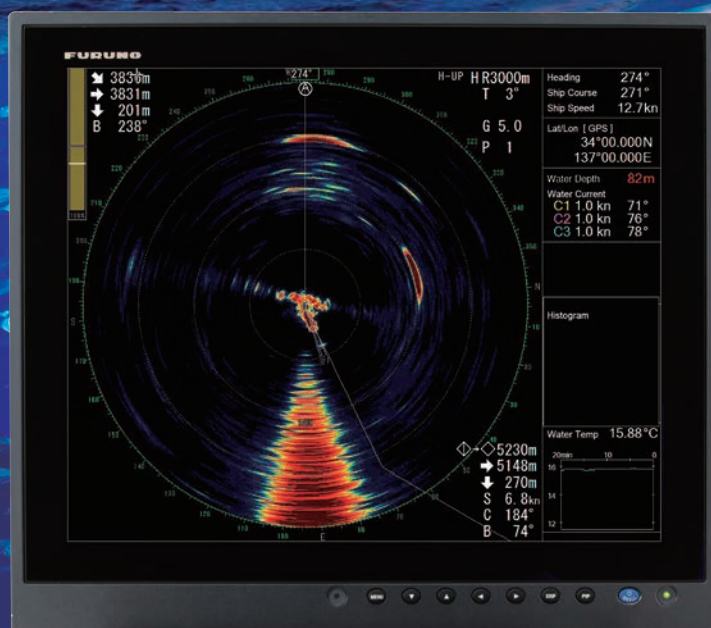
Photo: 19" Marine Display MU Series Monitor (Customer Supply)
