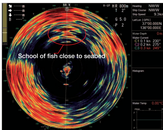
(800 m range) A school of fish close to the seabed can be distinguished clearly.
